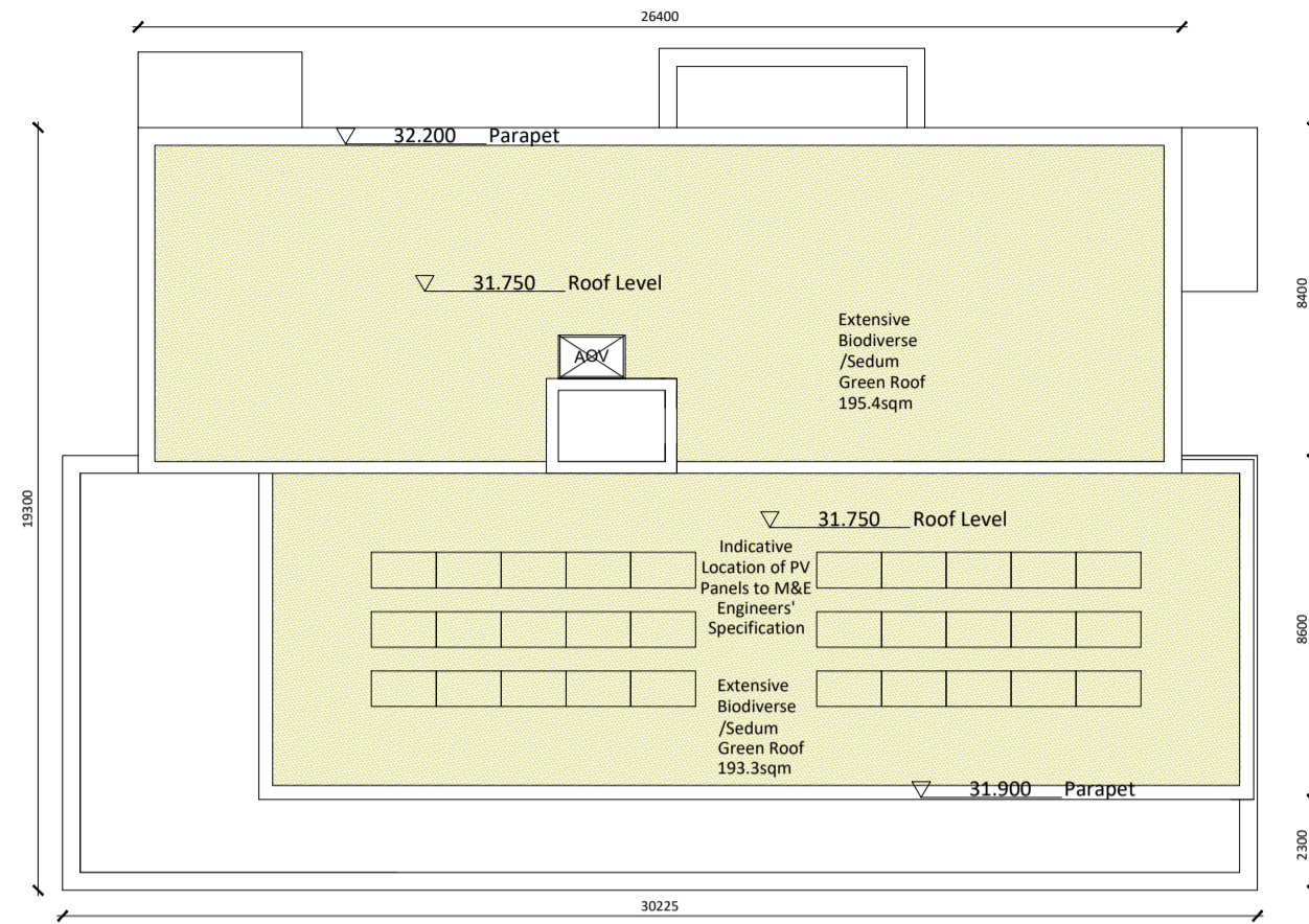
Roof Plan
